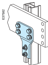
Prefabricated connection 1000 A.
