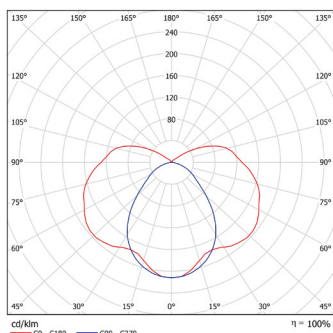
ALHAMA 136 LED-T8 PC C2
