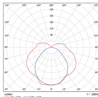
ALHAMA 236 LED-T8 PC C2
